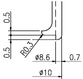
C部詳細 (2:1)
